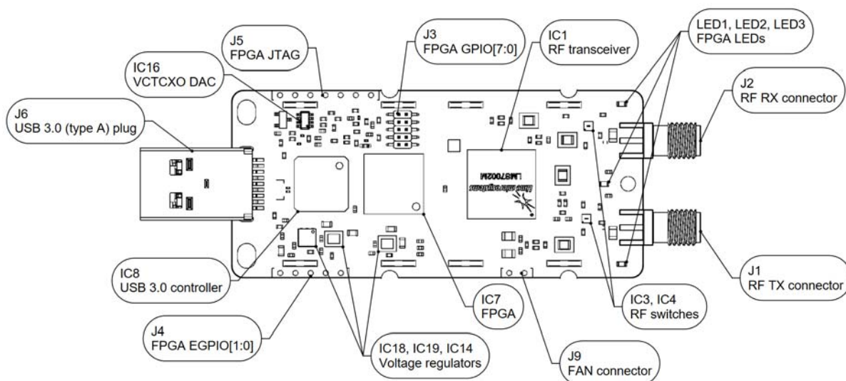
Figure 4: LimeSDR Mini v2.3 board top connectors and main components
