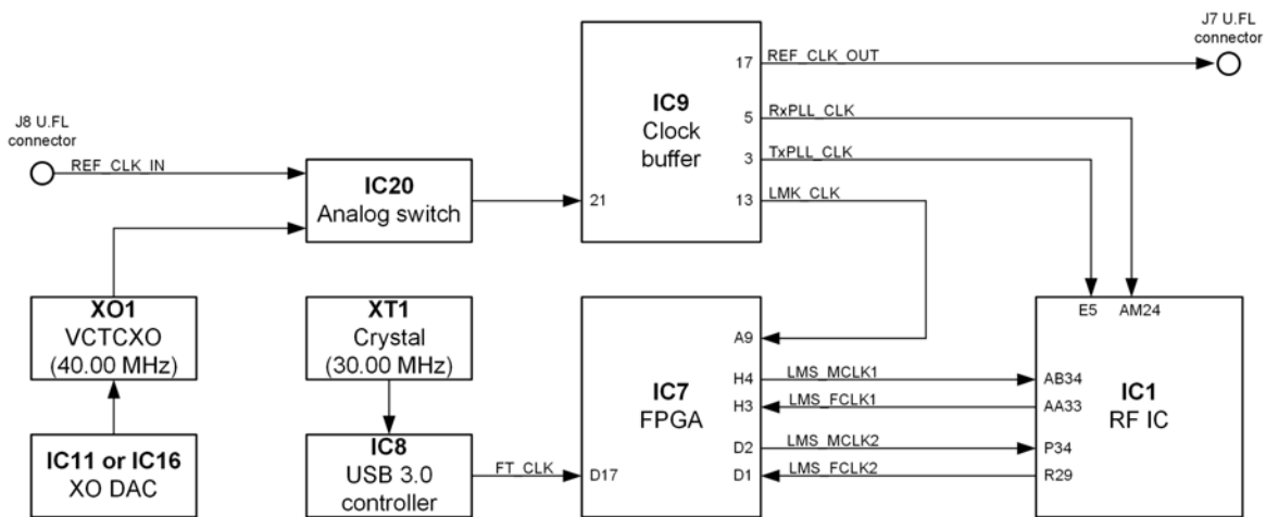
Figure 9: LimeSDR Mini v2.3 board clock distribution block diagram
