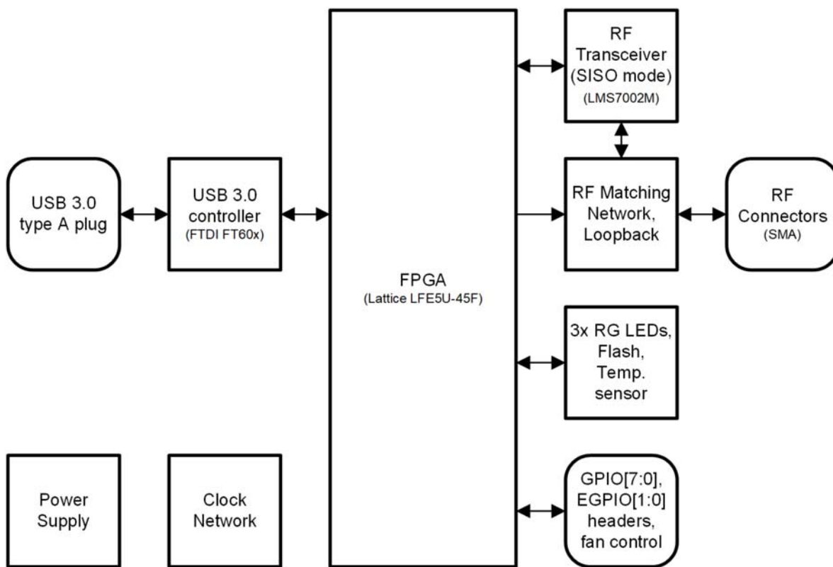
Figure 3: LimeSDR Mini v2.3 Development Board Block Diagram
