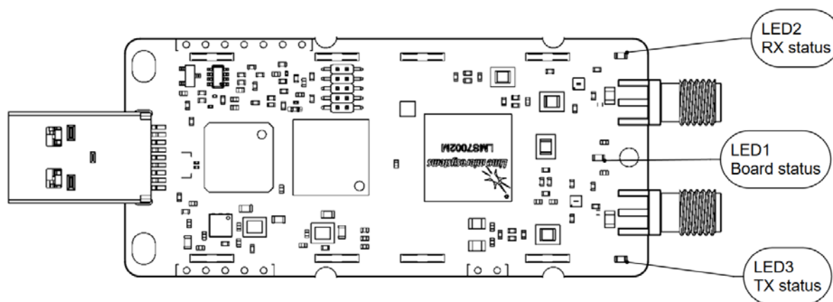
Figure 7: LimeSDR Mini v2.3 indication LEDs (top and bottom)
