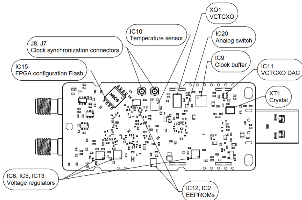
Figure 5: LimeSDR Mini v2.3 board bottom connectors and main components
