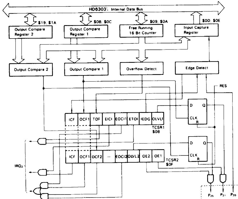
Figure 22 Timer 1 Block Diagram
