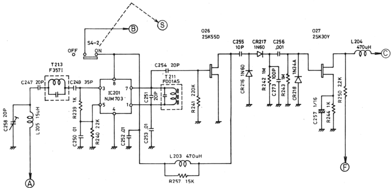
Figure 5-1 Noise Blanking Circuit
