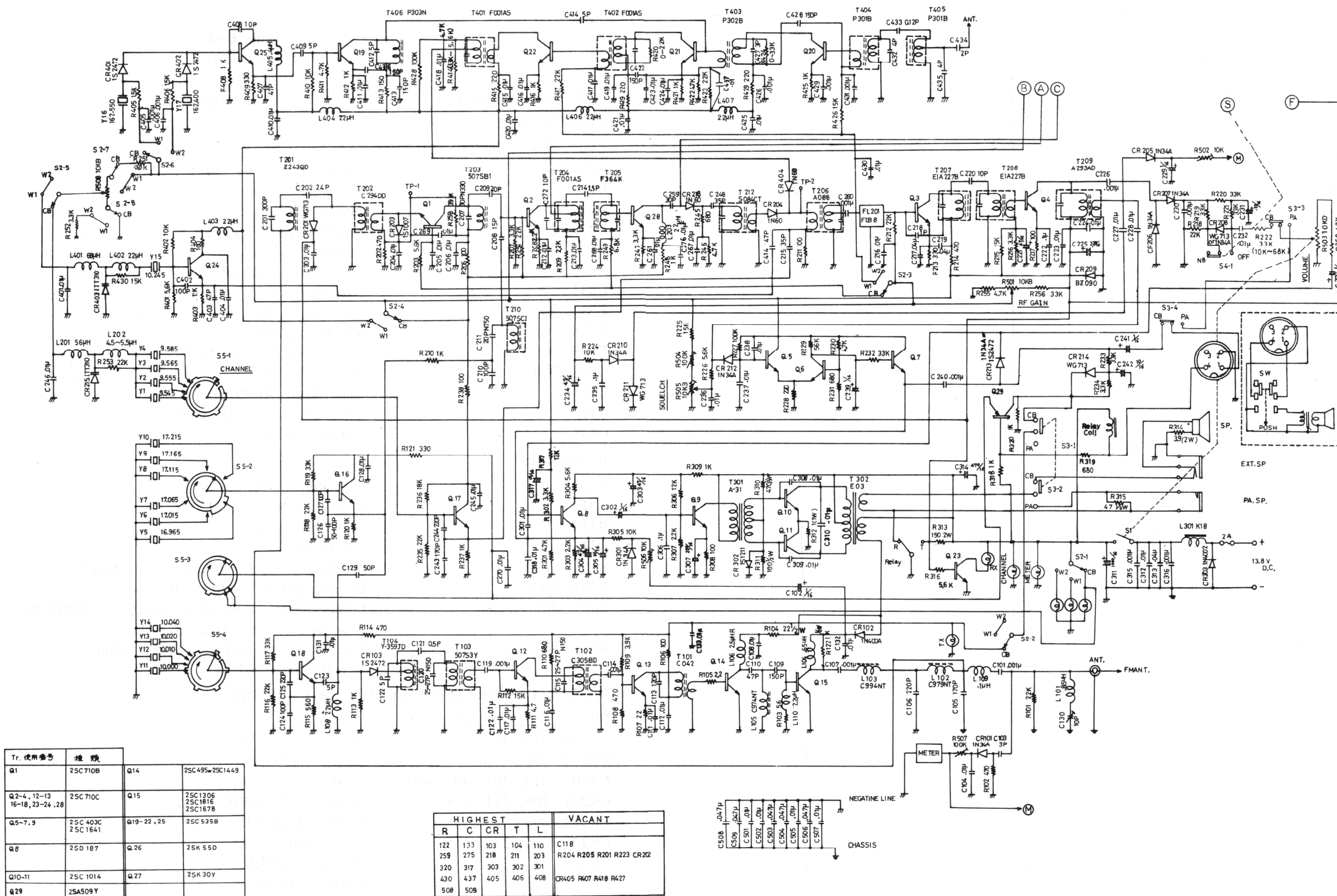
Figure 5-3 Schematic
