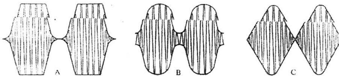
Waveforms Figure 1
