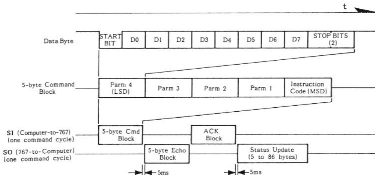
CAT SYSTEM TIMING CHART
