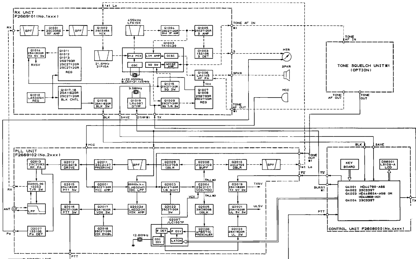
#1 RX PLL AND CONTROL COMPONENT VARIATIONS
