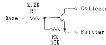
DTA123YU CIRCUIT DIAGRAM
