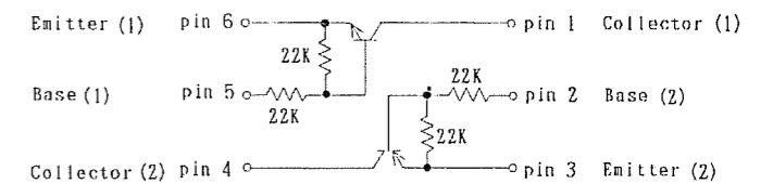
IMD2 CIRCUIT DIAGRAM
