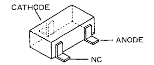
1SS294 (A9) (D3002)
