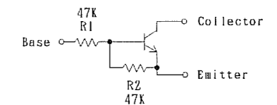
DTC144EU CIRCUIT DIAGRAM
