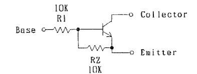
DTC114EU CIRCUIT DIAGRAM
