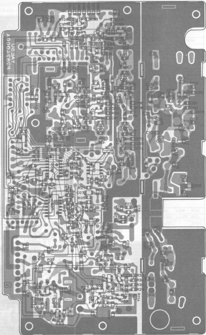
(reverse view of "chip-only" side)
