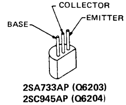
(obverse view of "component" side)
