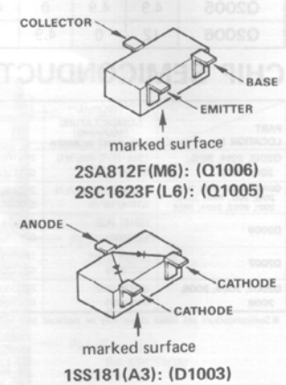
(reverse view of "IC" side)
