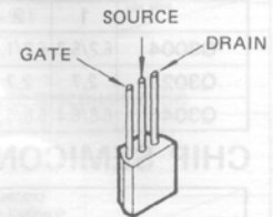
2SK192A-GR (Q4013)
