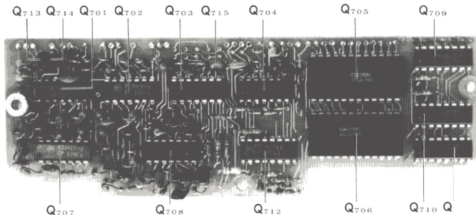
PLL CONTROL UNIT
