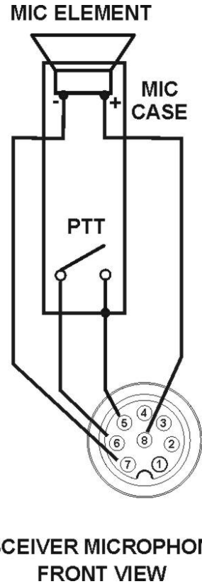
Figure 2-3. Recommended mic cable wiring.
