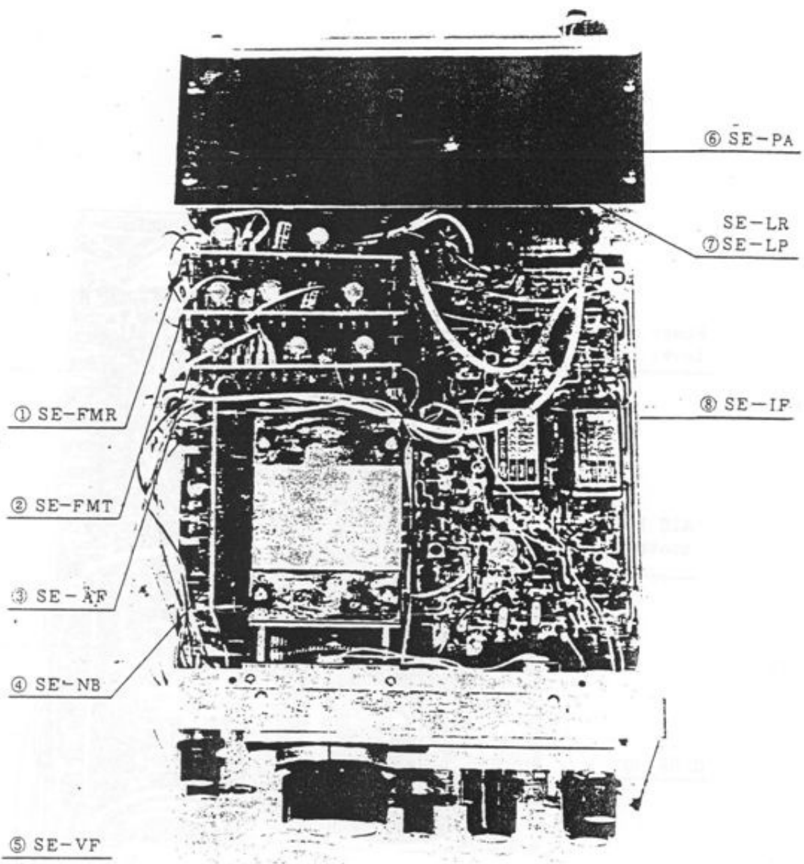
TOP VIEW
