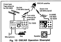
Fig. 10 OSCAR Operation (Example)
