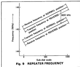
Fig. 9 REPEATER FREQUENCY
