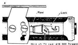
Fig. 6 Installing the Set on the Car
