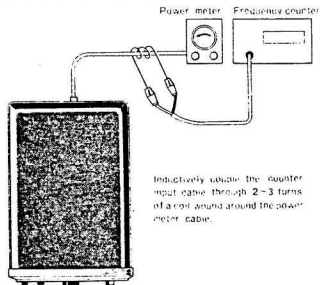
Fig. 11 Adjusting TX Section
