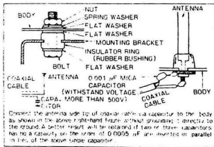
Fig. 5 Installation on the Positive Grounded Car
