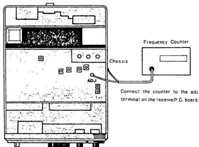
Fig. 10 Adjusting RX Section
