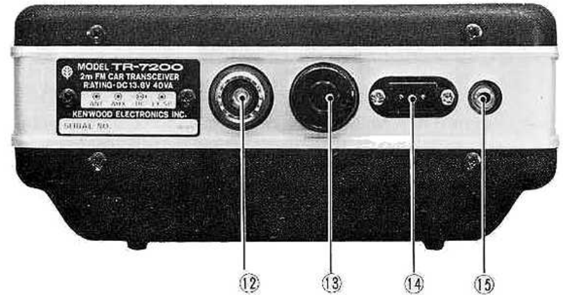
Fig. 2. Rear Panel
