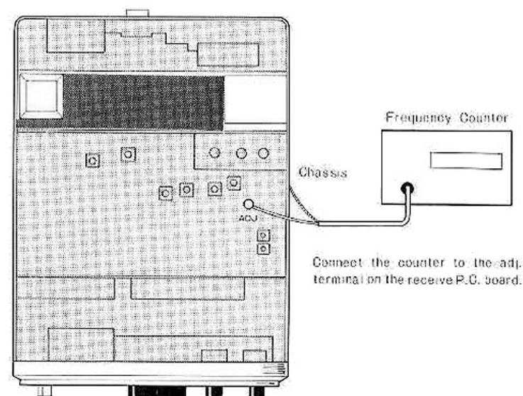
Fig. 10. Adjusting RX Section
