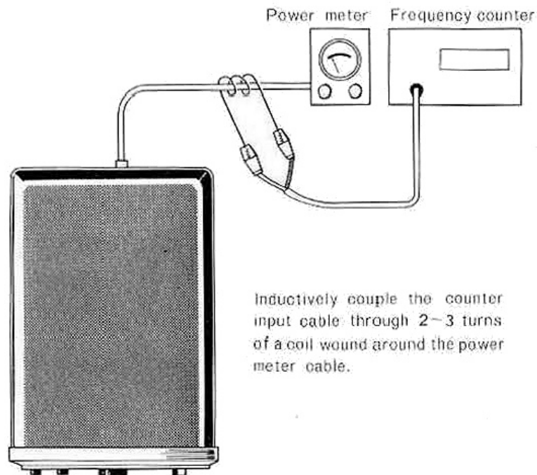
Fig. 11. Adjusting TX Section
