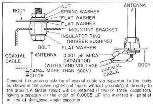
Fig. 5. Installation on the Positive Grounded Car
