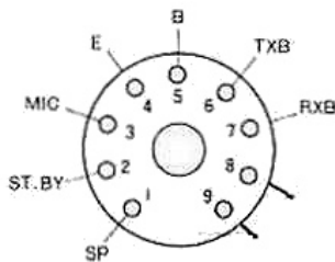
Fig. 9. AUX Connector Configuration
