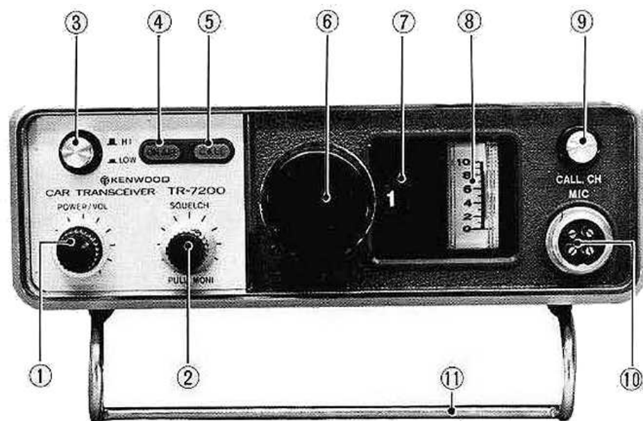
Fig. 1. Front Panel
