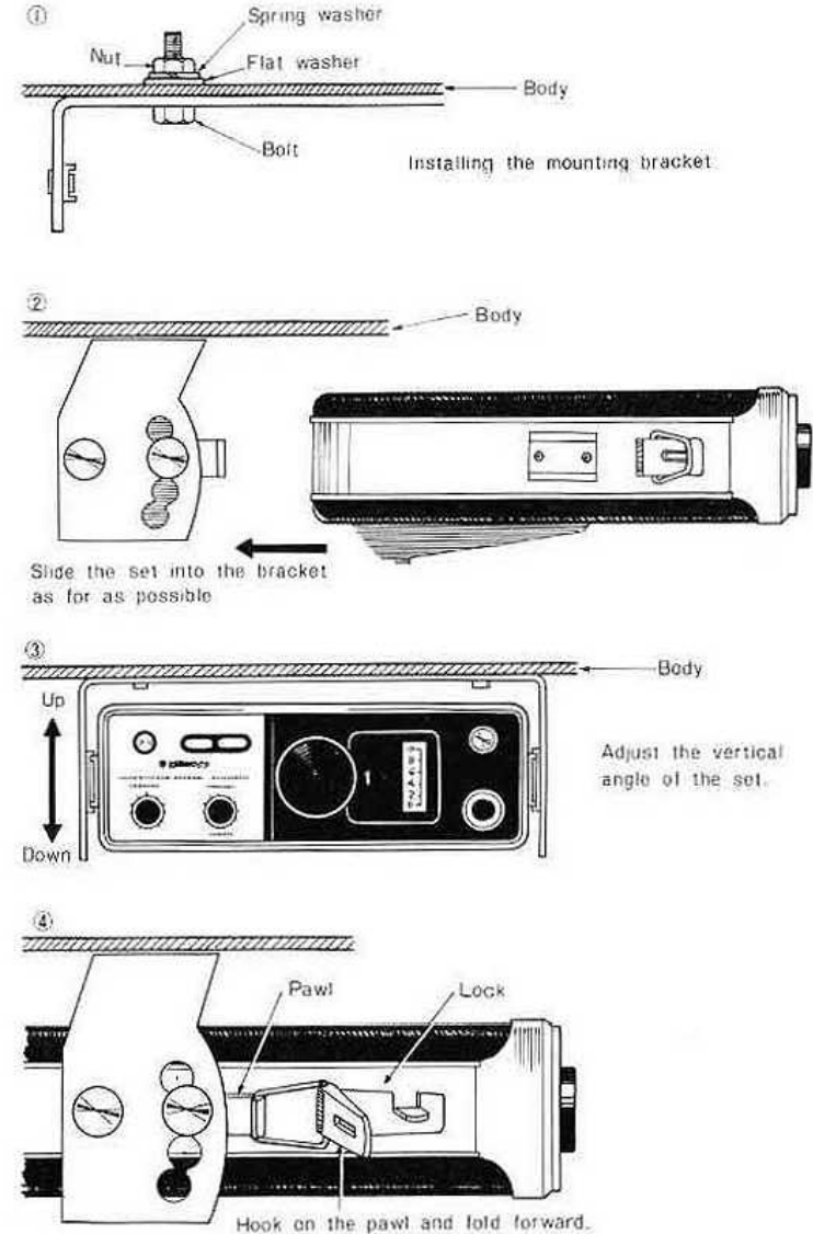
Fig. 6. Installing the Set on the Car
