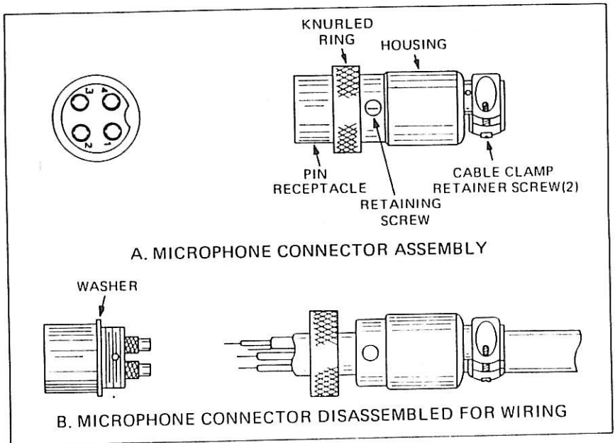
Fig. 4. Microphone plug wiring.
