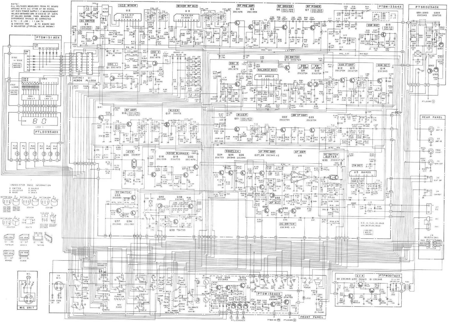
SCHEMATIC DIAGRAM : LARRY INTERNATIONAL 3
