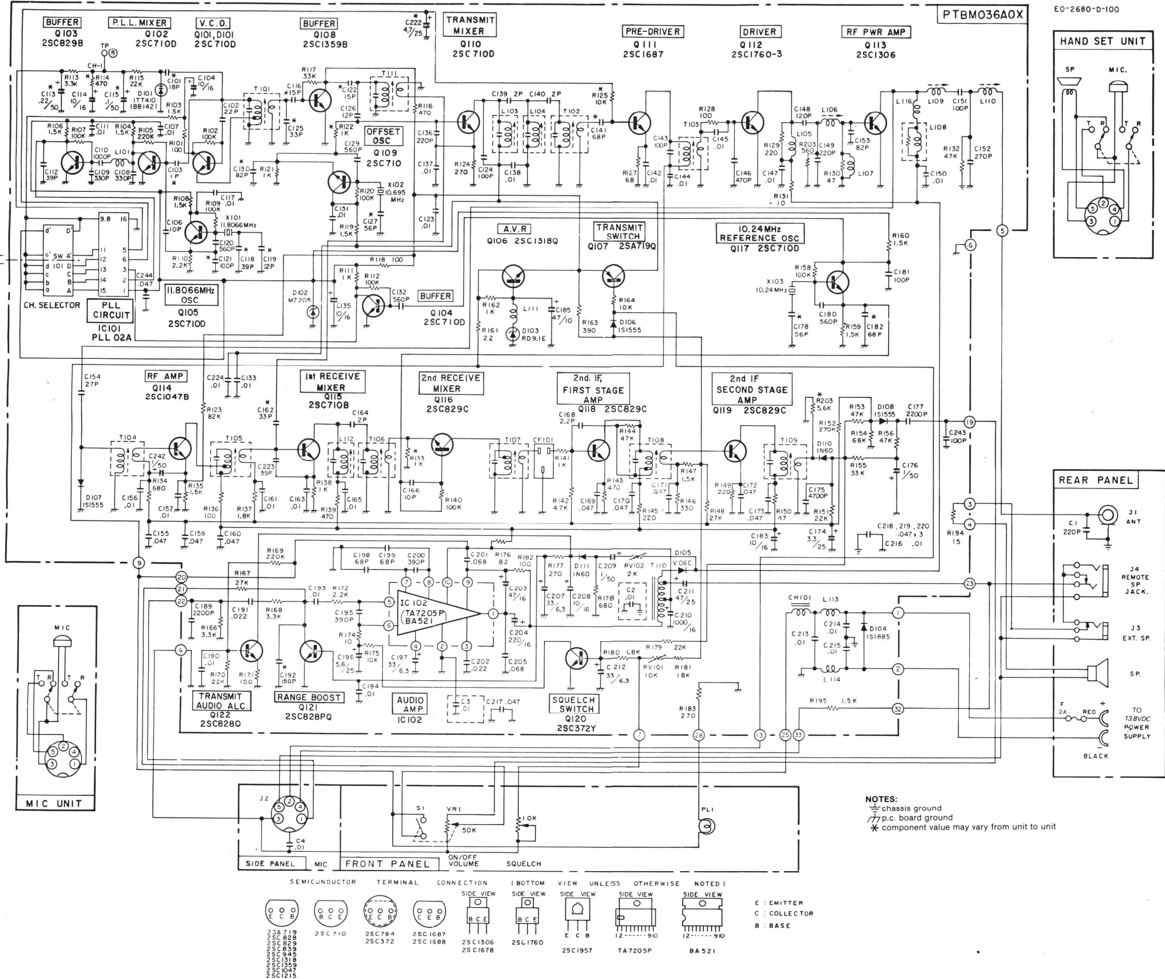
Figure 4-2. Schematic Diagram, Model 2680
