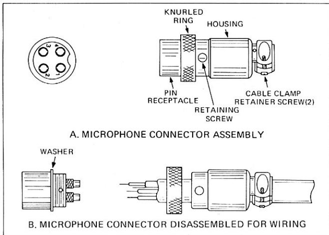
Fig. 4. Microphone plug wiring.
