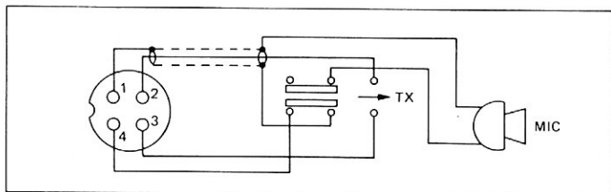
Fig. 3. 侍 samurai microphone schematic.
