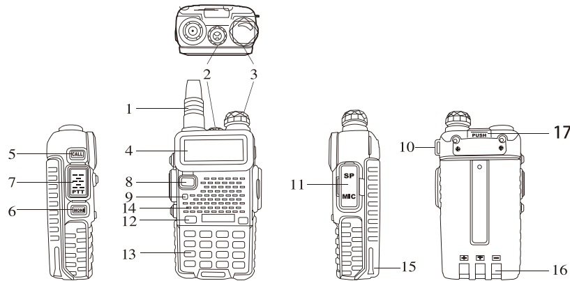
Figure 2.1. Baofeng UV-5RX3, overview
