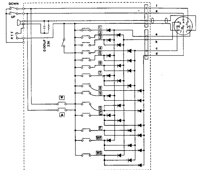
CIRCUIT DIAGRAM
