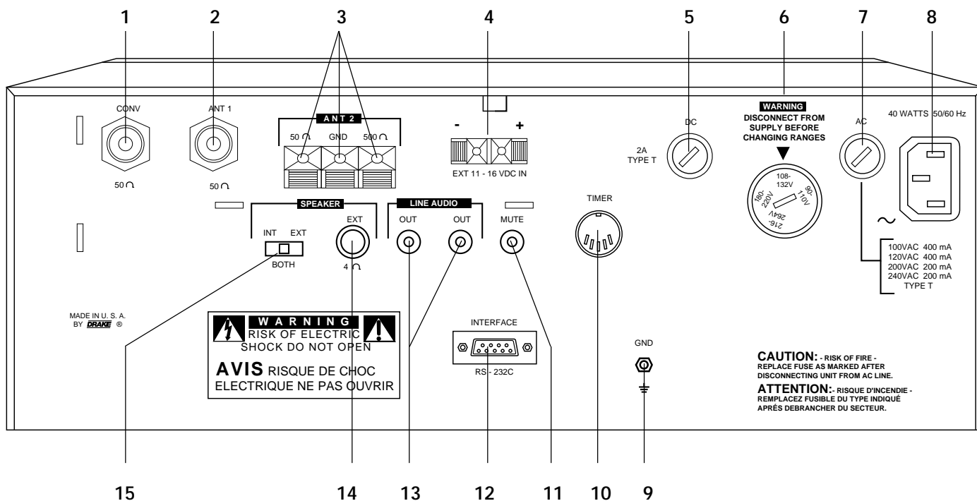
FIGURE 6 REAR PANEL
