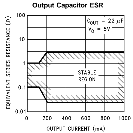
FIGURE 1. ESR Limits
