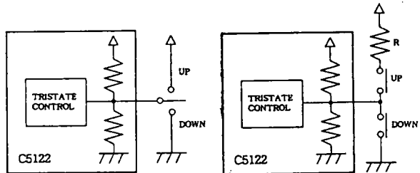
(Detent SW interface) (Push, up/down SW interface)
