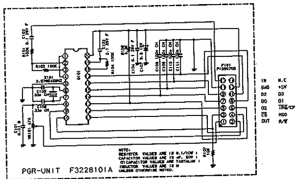
FRC-6 Circuit Diagram
