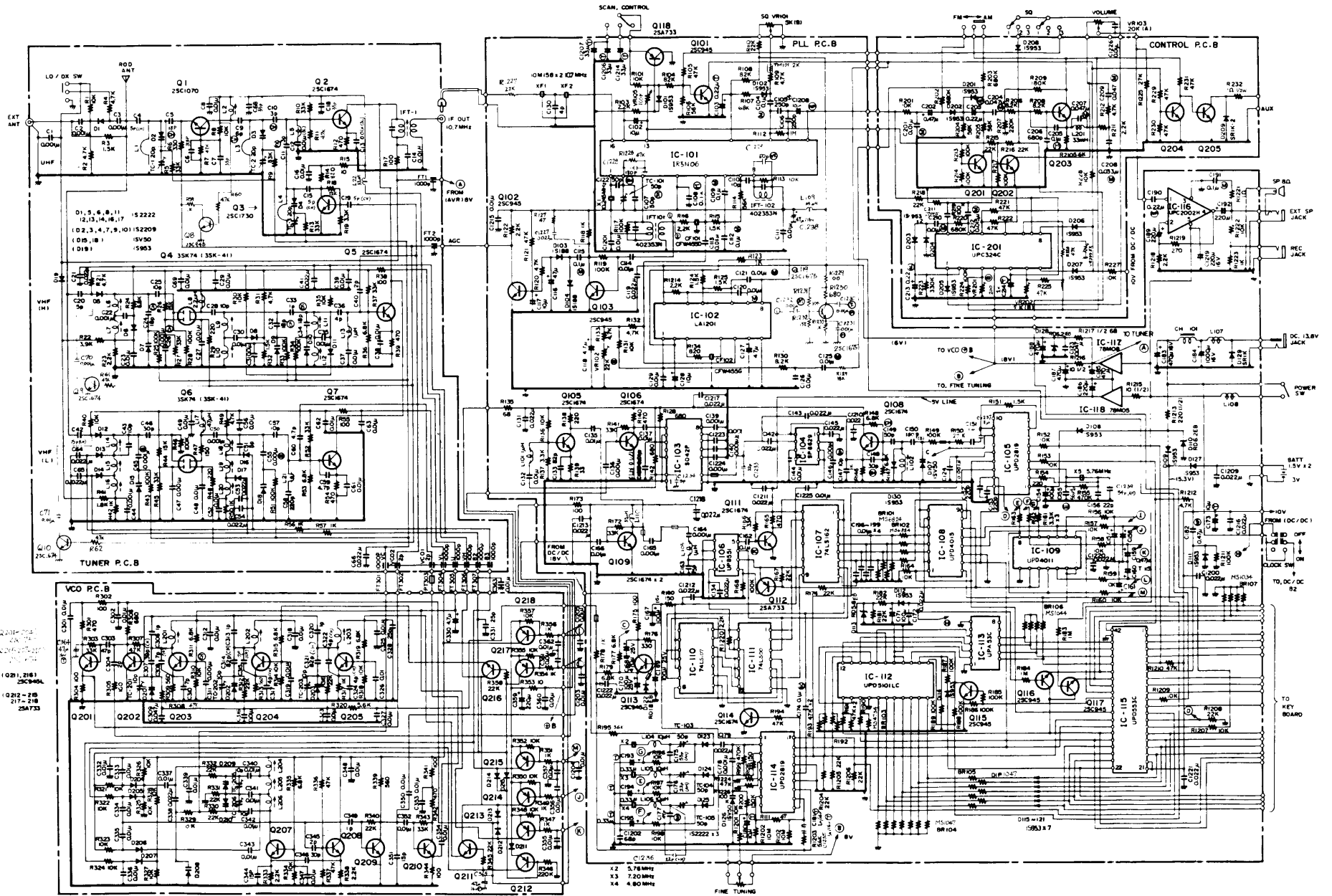
SCHMATIC DIAGRAM (PLL, TUNER, VCO, CONTROL) Fig. 5-1
