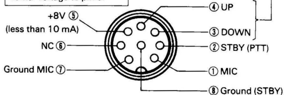
MIC connector < Front panel view >
