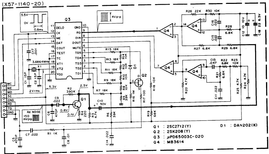
MU-1 SCHEMATIC DIAGRAM
