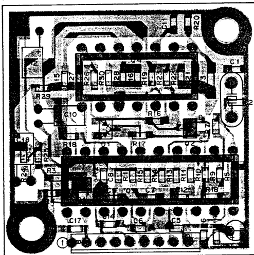
MU-1 PC BOARD VIEW (X57-1140-20) Component side view
