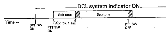
Fig. b. Offset mode (TM-3530A/2570A/2550A/2530A)
