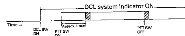
Fig. c. Offset mode (TM-2550E)
