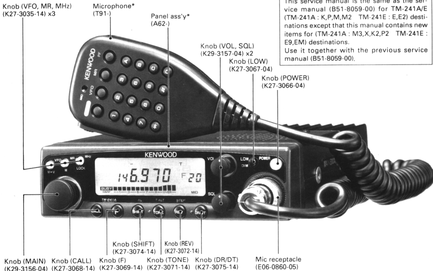
Photo is TM-241A. * Refer to parts list on page 15.
