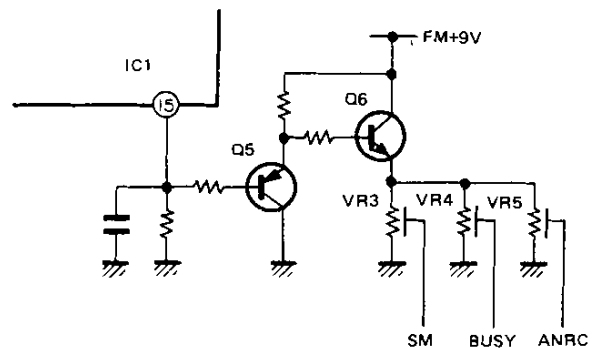
Fig. 4 S-meter circuit (FM-Wide)
