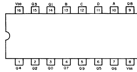
μPD4028BG IC5 (BCD TO DECIMAL DECODER)
