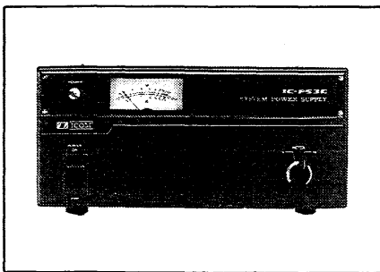
IC-PS30 AC POWER SUPPLY (13.8 V DC, 25 A)
