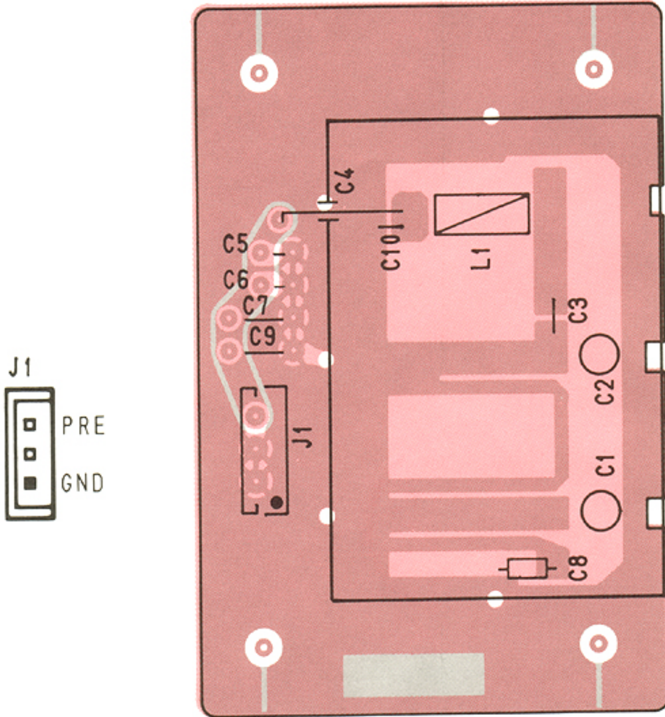
FILTER UNIT
