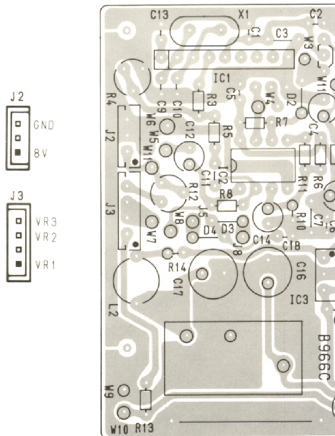
DC-DC UNIT (#02)
