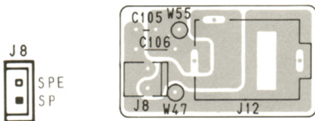
JACK UNIT
