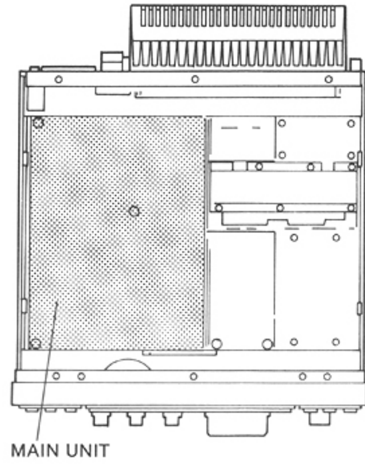
(TOP VIEW)
