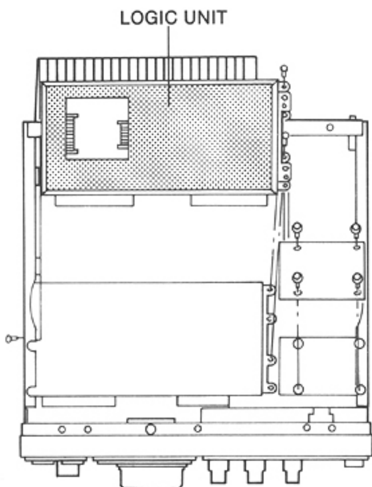
(BOTTOM VIEW)
