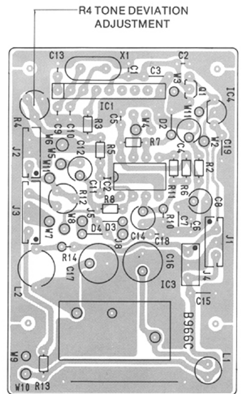
DC-DC UNIT (#02 Only)
