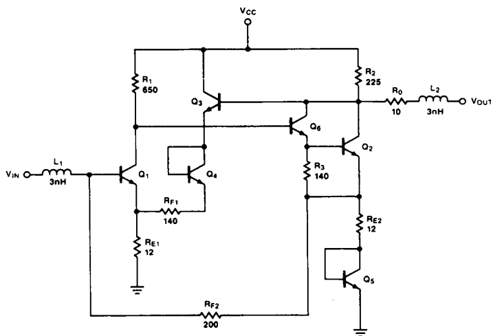
Figure 15. Schematic Diagram
