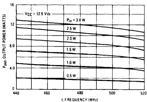
FIGURE 16 – OUTPUT POWER versus FREQUENCY
