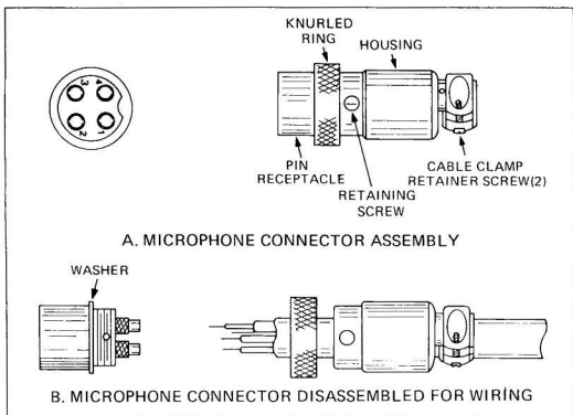
Fig. 4. Microphone plug wiring.
