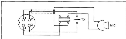
Fig. 3. SUPER STAR 3900 microphone schematic.
