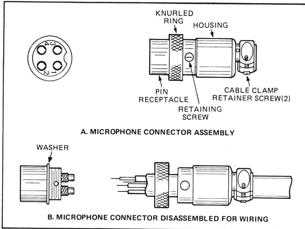
Fig. 4. Microphone plug wiring.
