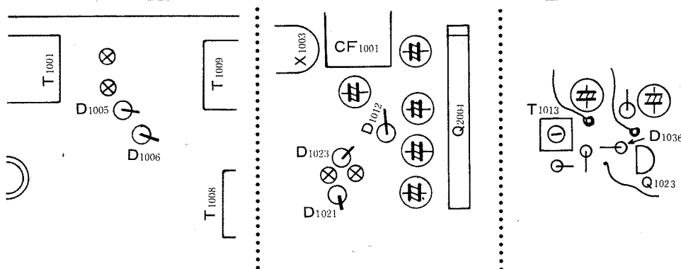
RECEIVER SECTION ALIGNMENT POINTS
