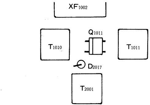
TRANSMITTER SECTION ALIGNMENT POINTS
