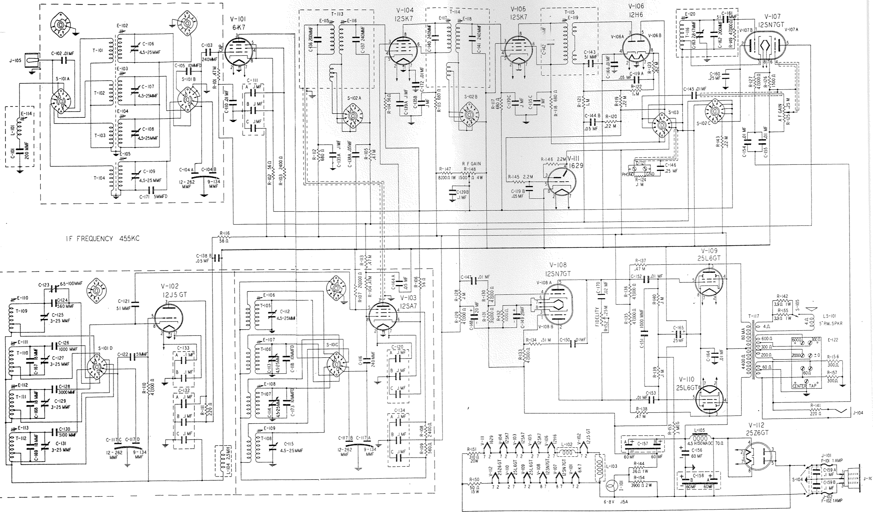
Fig. 11 Schematic Diagram Scott Marine Radio Receiver
