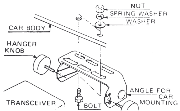
Fig. 2 Mounting method
