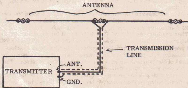
Fig. 3. Half-Wave Dipole Antenna.
