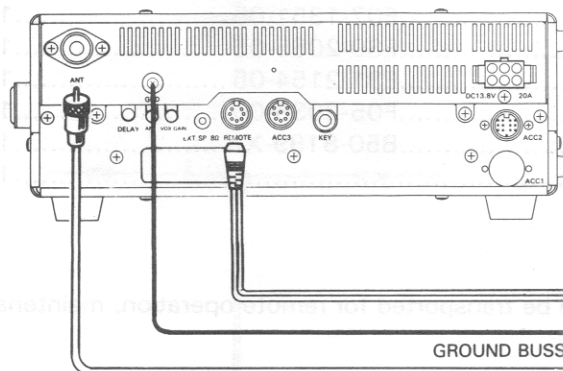
EXCITER, TS-140S/680S
