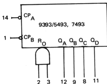
LOGIC SYMBOL
