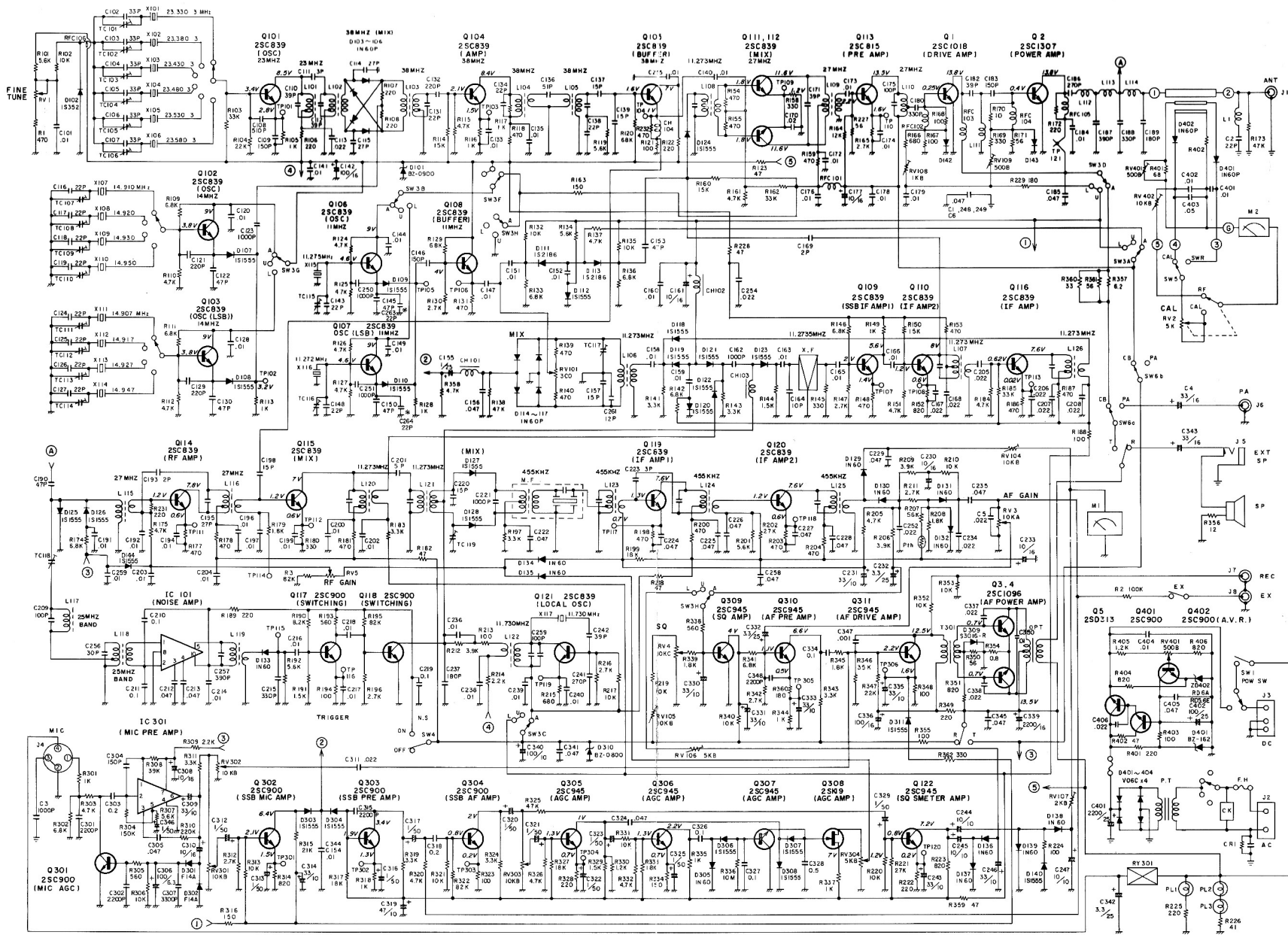
SCHEMATIC DIAGRAM OF 13-898B
