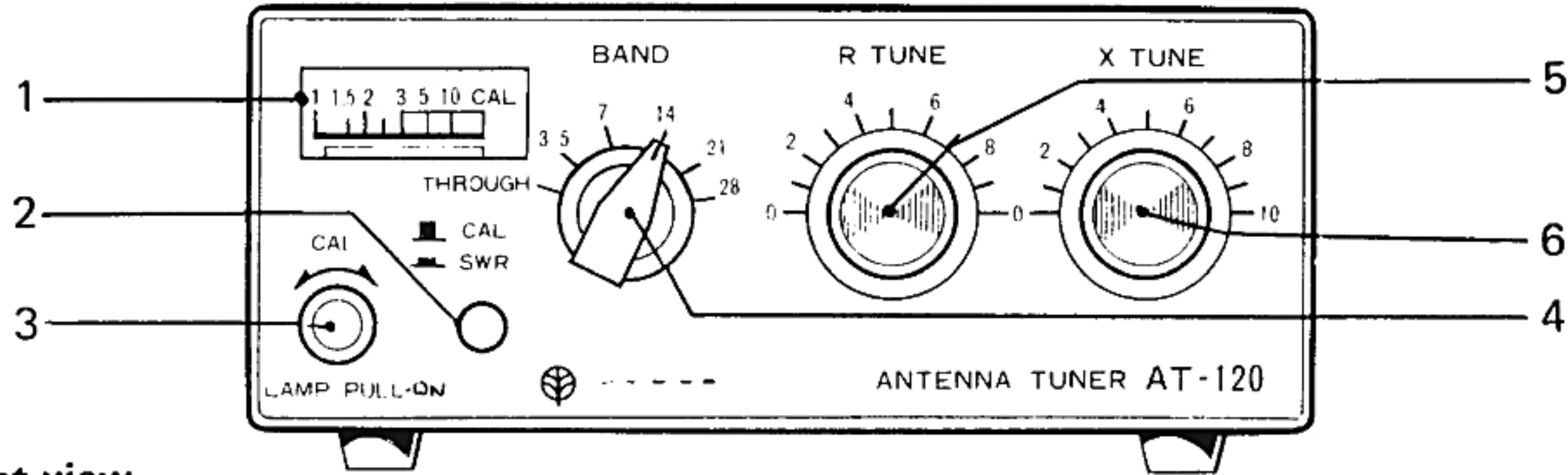
Figure 3. Front view
